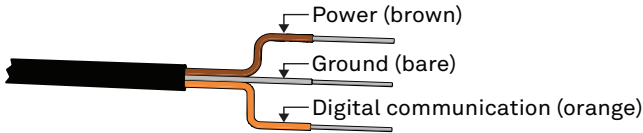
Figure 2 Pigtail wiring
